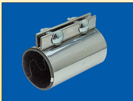
Pipe connectors for pneumatic conveying
