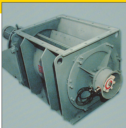
Rotary valves drop or blow through
