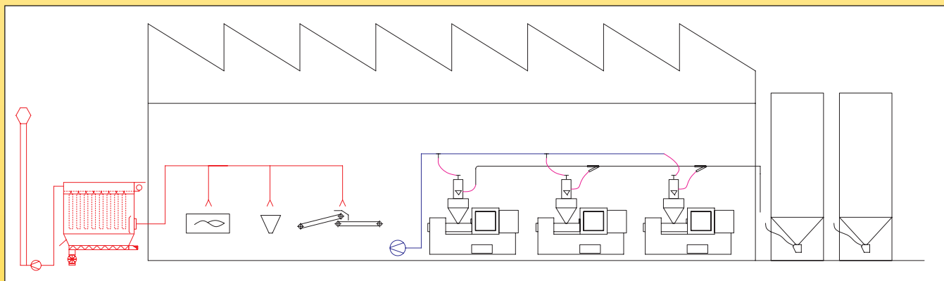
PNEUMATIC CONVEYING SYSTEMS FOR FEEDING RAW MATERIALS IN THE PLASTIC INDUSTRIES. DEDUSTING DIFFERENT WORK PLACES
